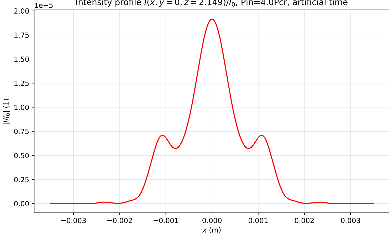
Intensity profile I(x, y = 0, z = 2.149)/I_0 , P_{in}=4.0P_{cr} , artificial time
